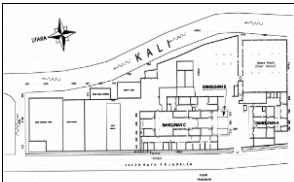
Gambar 7. Site Plan
