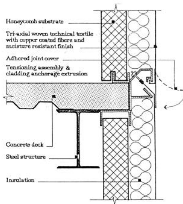
Sistim Pengikat Cladding Technical Textiles
