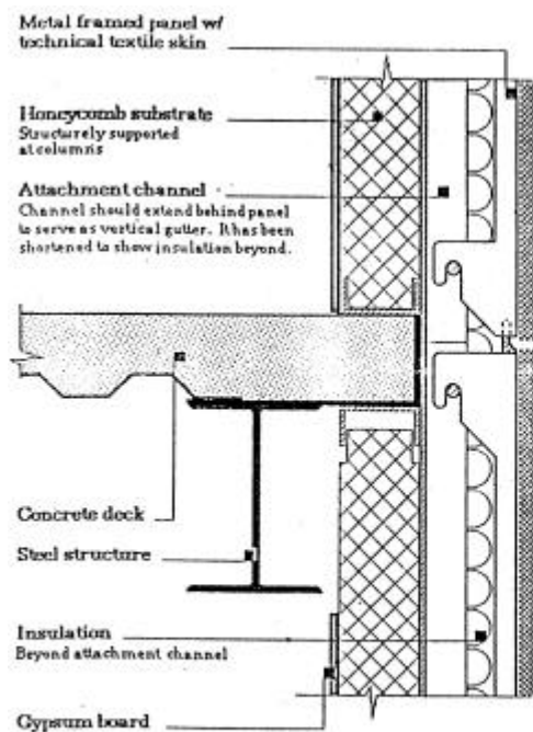
Sistim Pengait Cladding Technical Textiles (POHL Europanel System)
