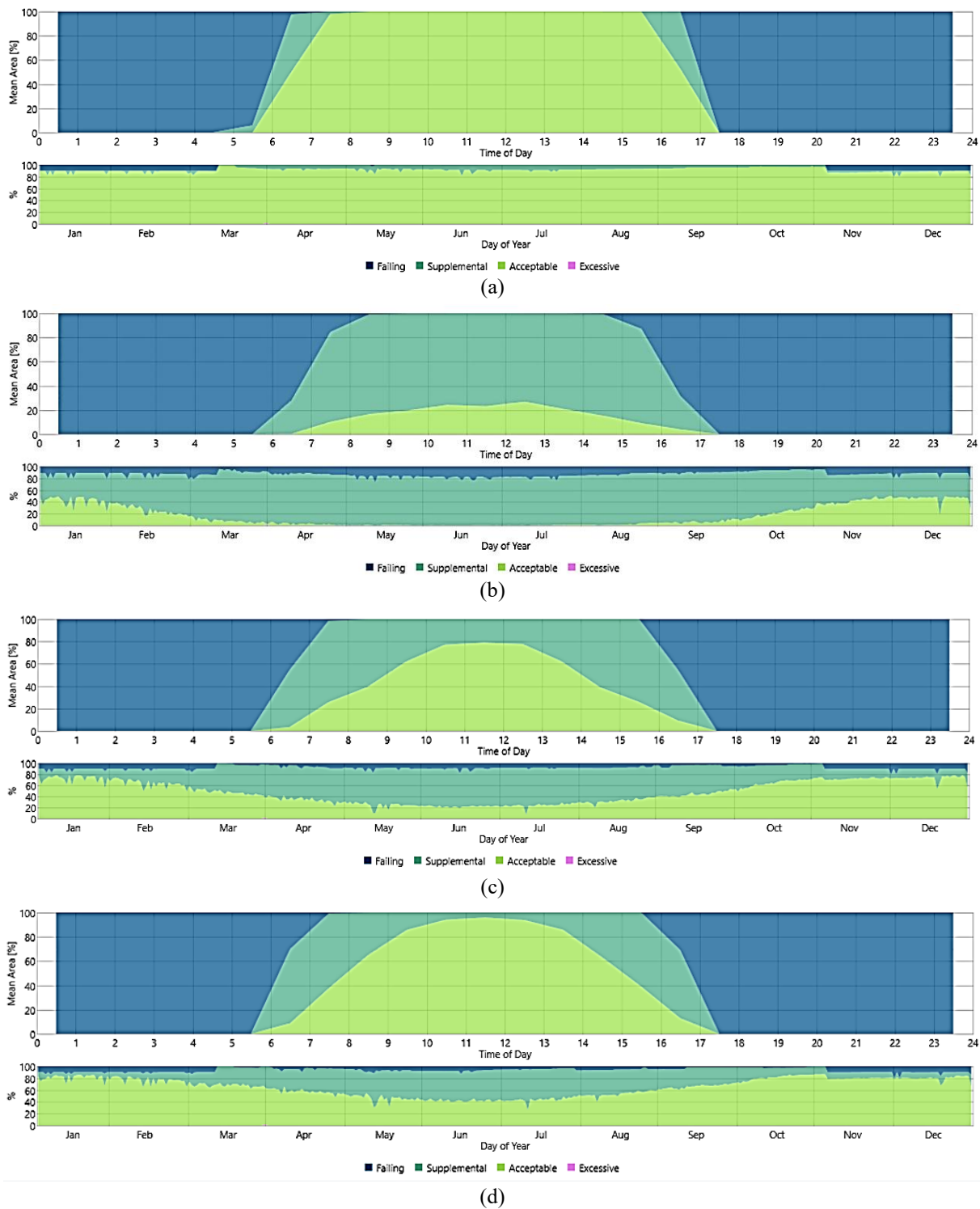
Fig. 11. The temporal graph of Useful Daylight Illuminance of mezzanine floor of loft office with (a) glazed facade and glazed facade and perforated screen facade with perforation percentages of (b) 20% (c) 30% and (d) 40%
